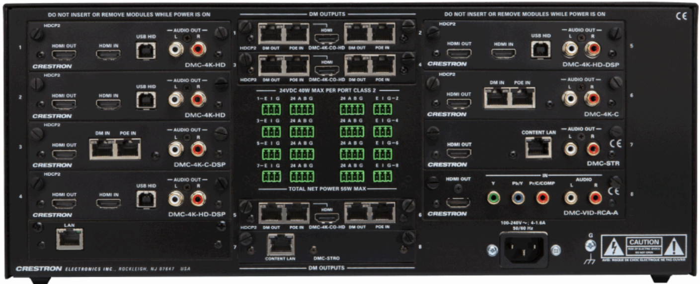
DM-MD8X8 – Rear view with I/O cards installed
