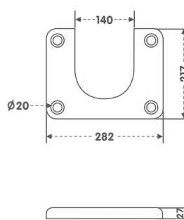
130 Slider Base Plate
