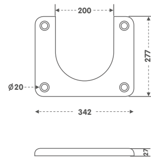
190 Slider Base Plate
