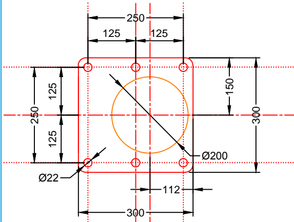
Typical Base Plate Detail
