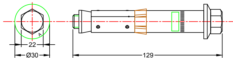
Typical Fixing Detail - 20mm Undercut Anchor Bolt
